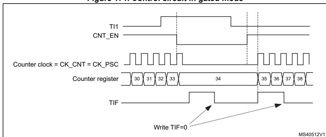
Figure 171. Control circuit in gated mode
