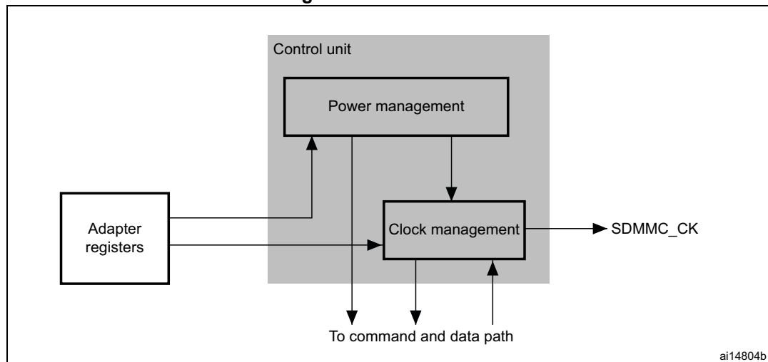
Figure 328. Control unit
