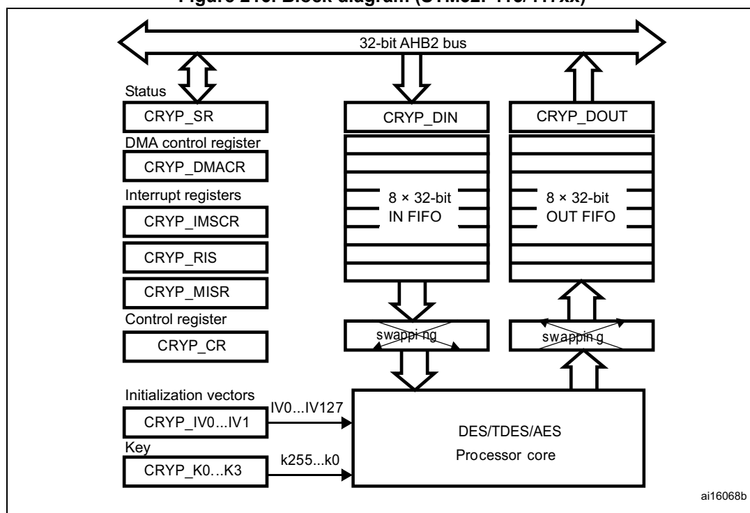
Figure 216. Block diagram (STM32F415/417xx)
